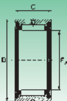
RNA 49..2RS
