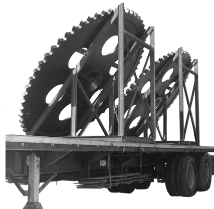
10 FT. DIAMETER ACCU-TORCH® FOR PAPER MILLS
